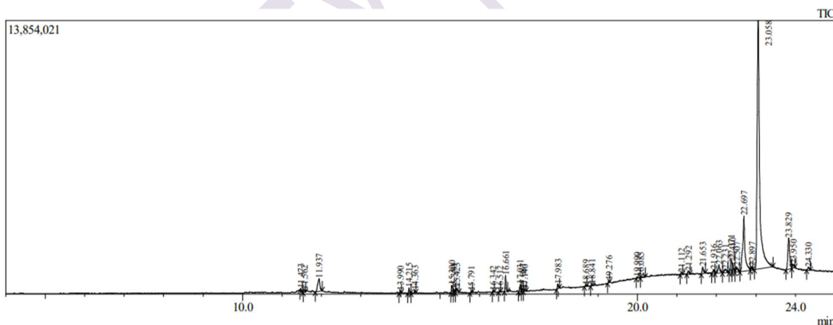
Figure 1. Chromatogram of Bauhinia purpurea root extract.
